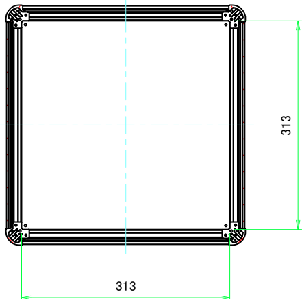
B-B (1:5.5)
