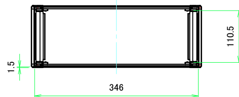
A-A (1:5.5)
