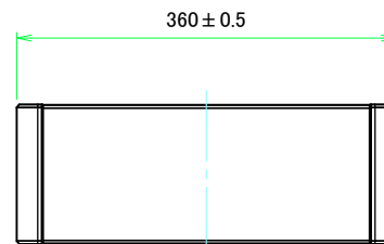
C view
