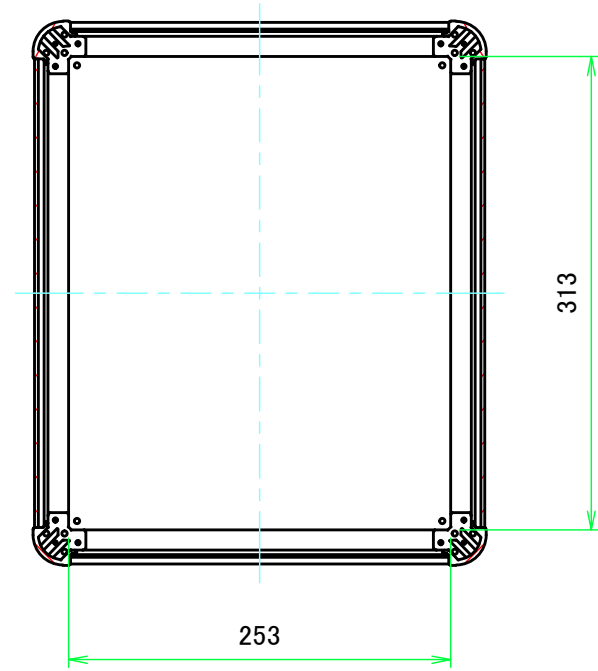
D view
