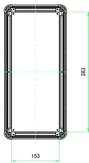
B-B (1:5)
