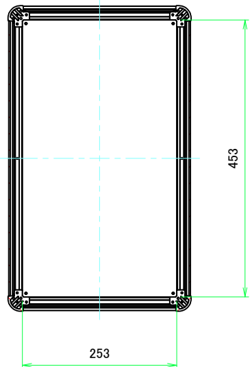
B-B (1:6)
