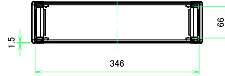
A-A (1:5.5)
