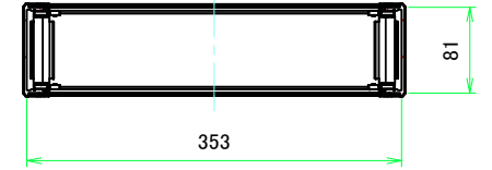
C-C (1:5.5)
