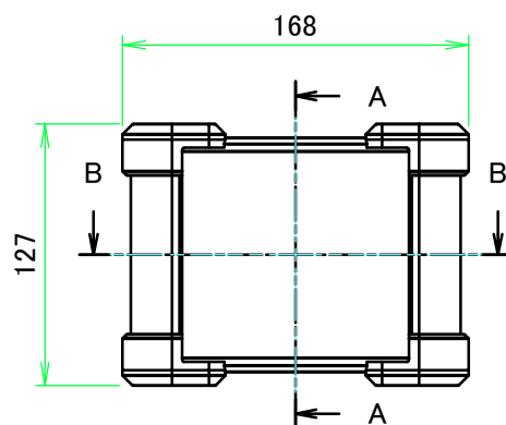
A view
