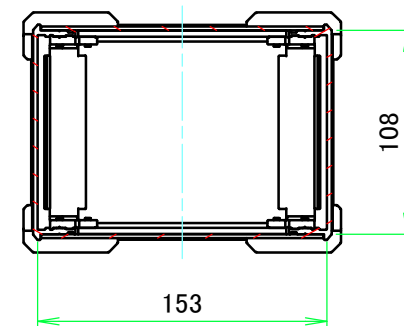
C-C (1:4)
