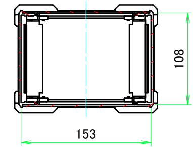
C-C (1:4.5)
