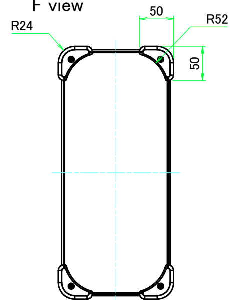
F view
