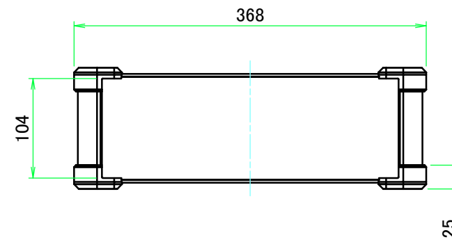
C view
