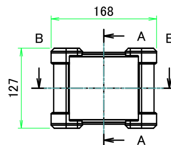
A view
