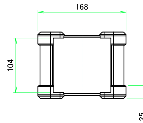
C view
