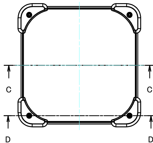
E view
