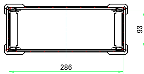
A-A (1:5.5)
