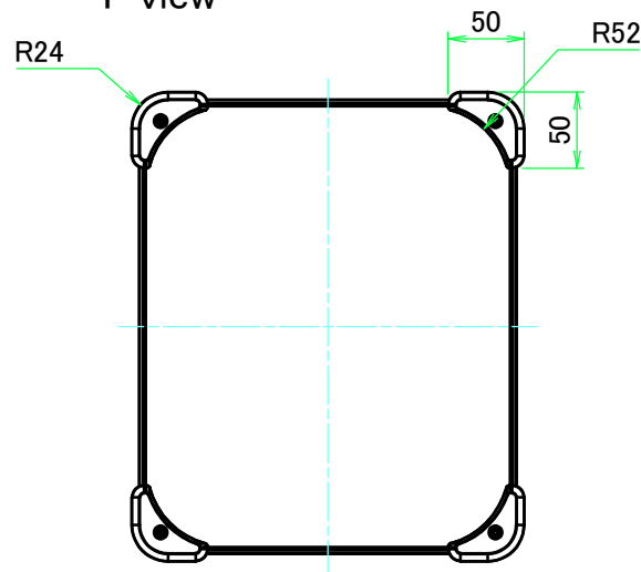
F view
