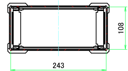
C-C (1:5.5)
