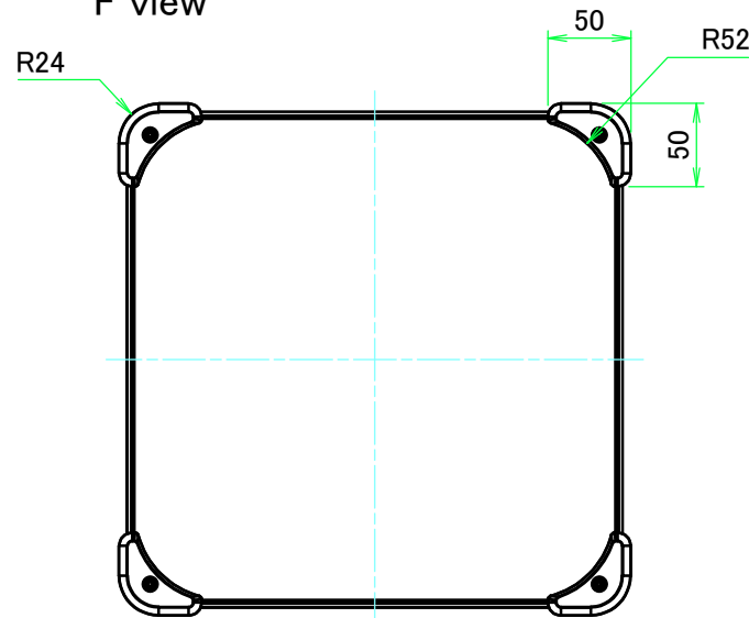
F view
