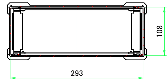
C-C (1:5)
