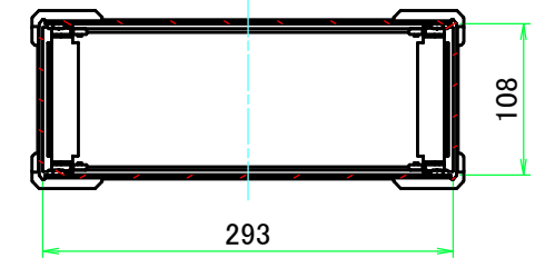
C-C (1:6)
