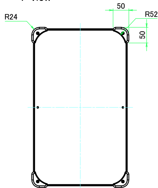
F view
