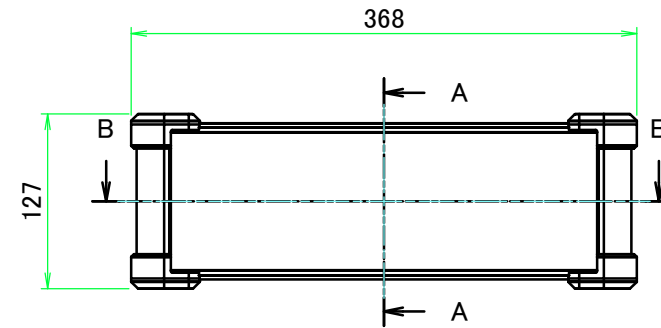
A view
