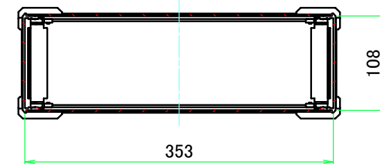
C-C (1:6)
