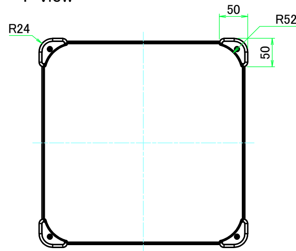
F view
