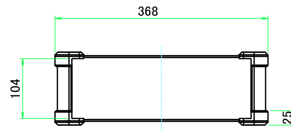
C view
