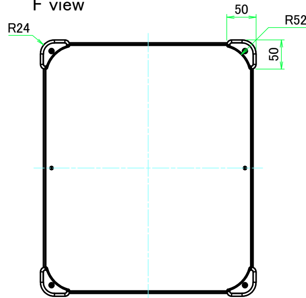
F view
