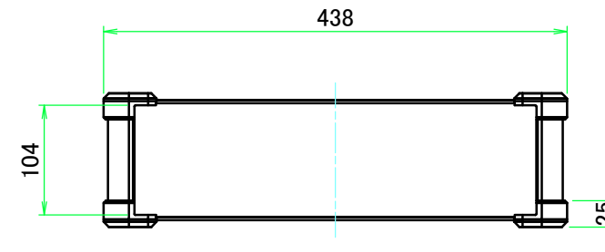
C view
