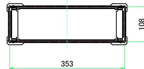
C-C (1:7)
