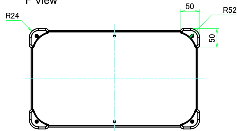
F view
