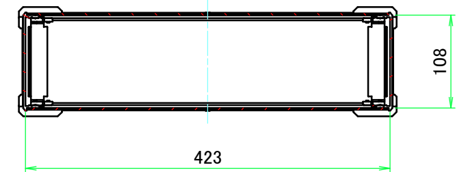
C-C (1:6)
