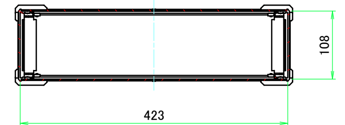
C-C (1:6)
