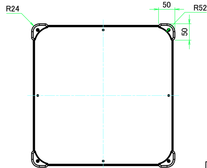
F view
