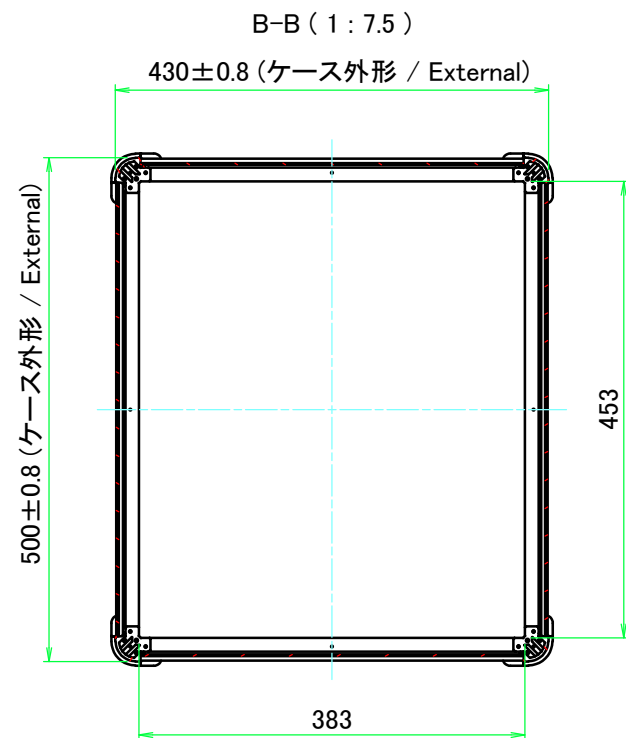
D view
