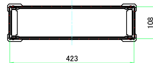
C-C (1:7.5)
