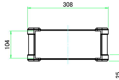
C view
