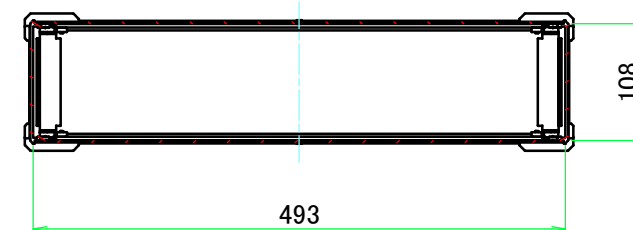
C-C (1:7)
