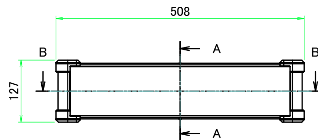
A view
