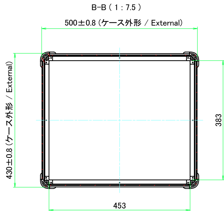
D view
