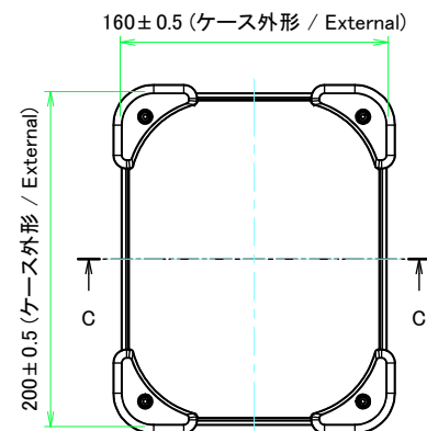
E view
