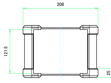
C view
