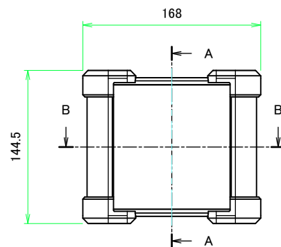
A view
