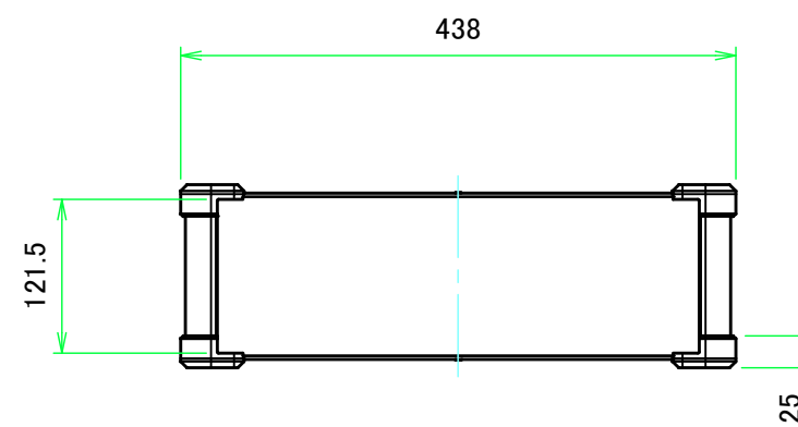
C view
