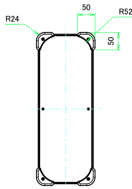
F view
