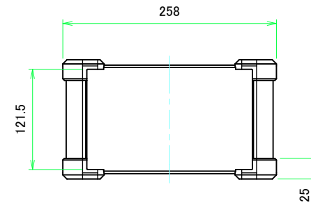
C view
