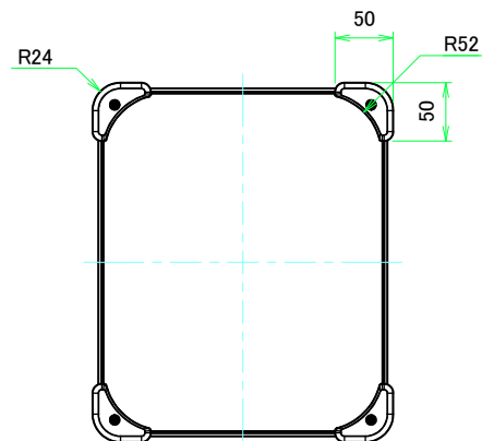
F view
