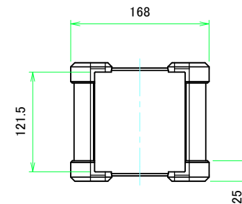
C view
