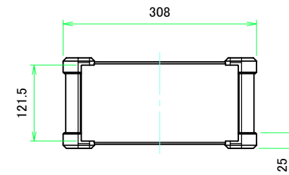
C view
