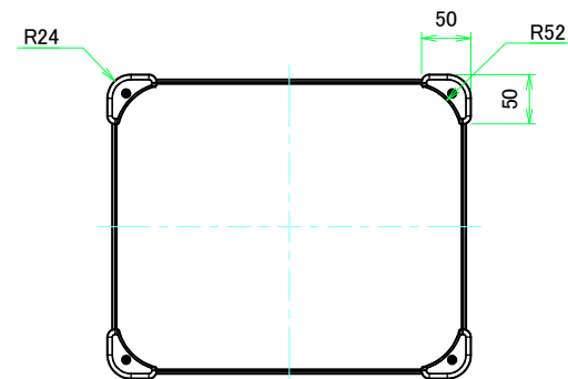
F view
