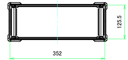
C-C (1:6)
