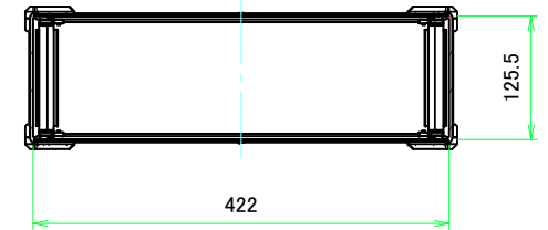
C-C (1:6)
