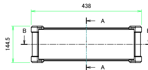
A view
