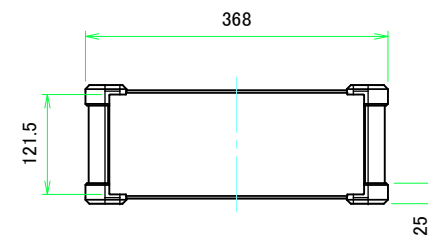
C view
