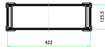
C-C (1:7)
