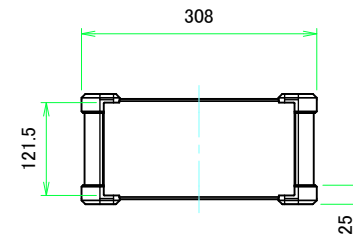
C view
