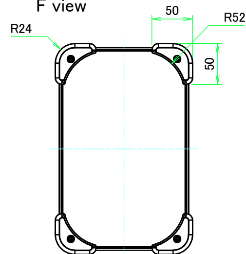
F view
