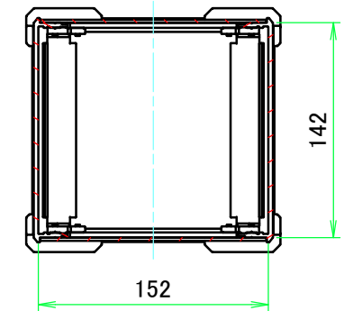
C-C (1:4.5)
