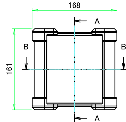
A view
