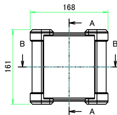
A view
