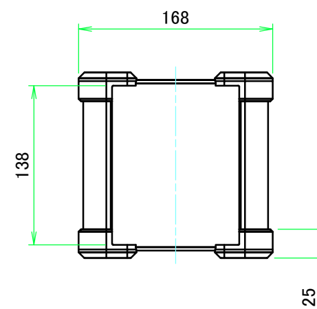
C view
