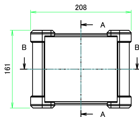
A view
