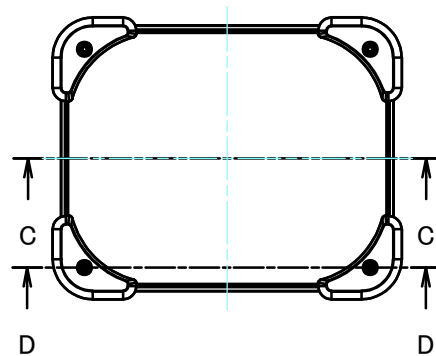
E view
