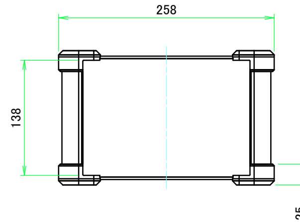
C view
