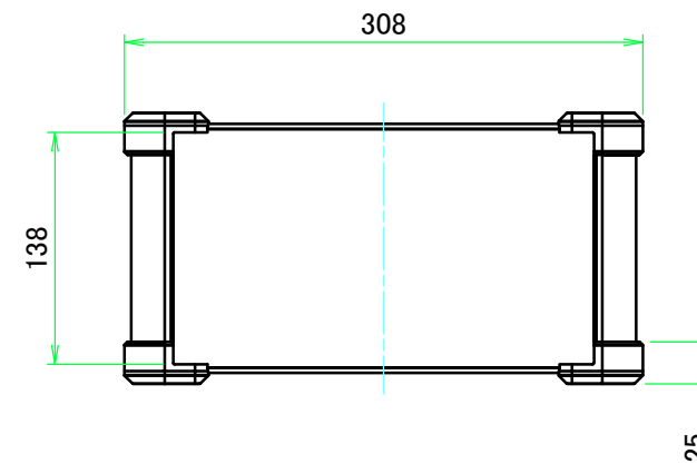
C view
