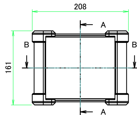
A view
