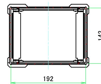
C-C (1:5)
