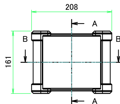
A view
