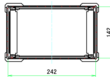
C-C (1:5)
