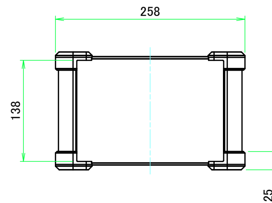
C view
