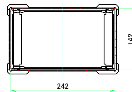
C-C (1:5)
