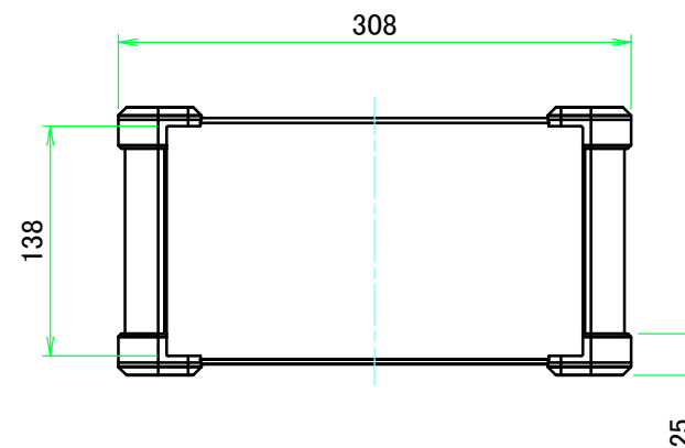
C view
