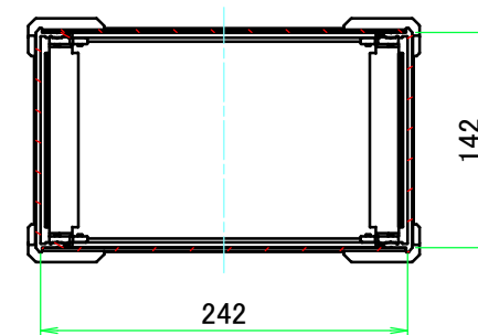
C-C (1:5.5)
