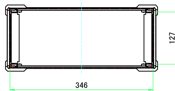
A-A (1:5.5)
