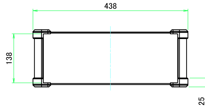
C view
